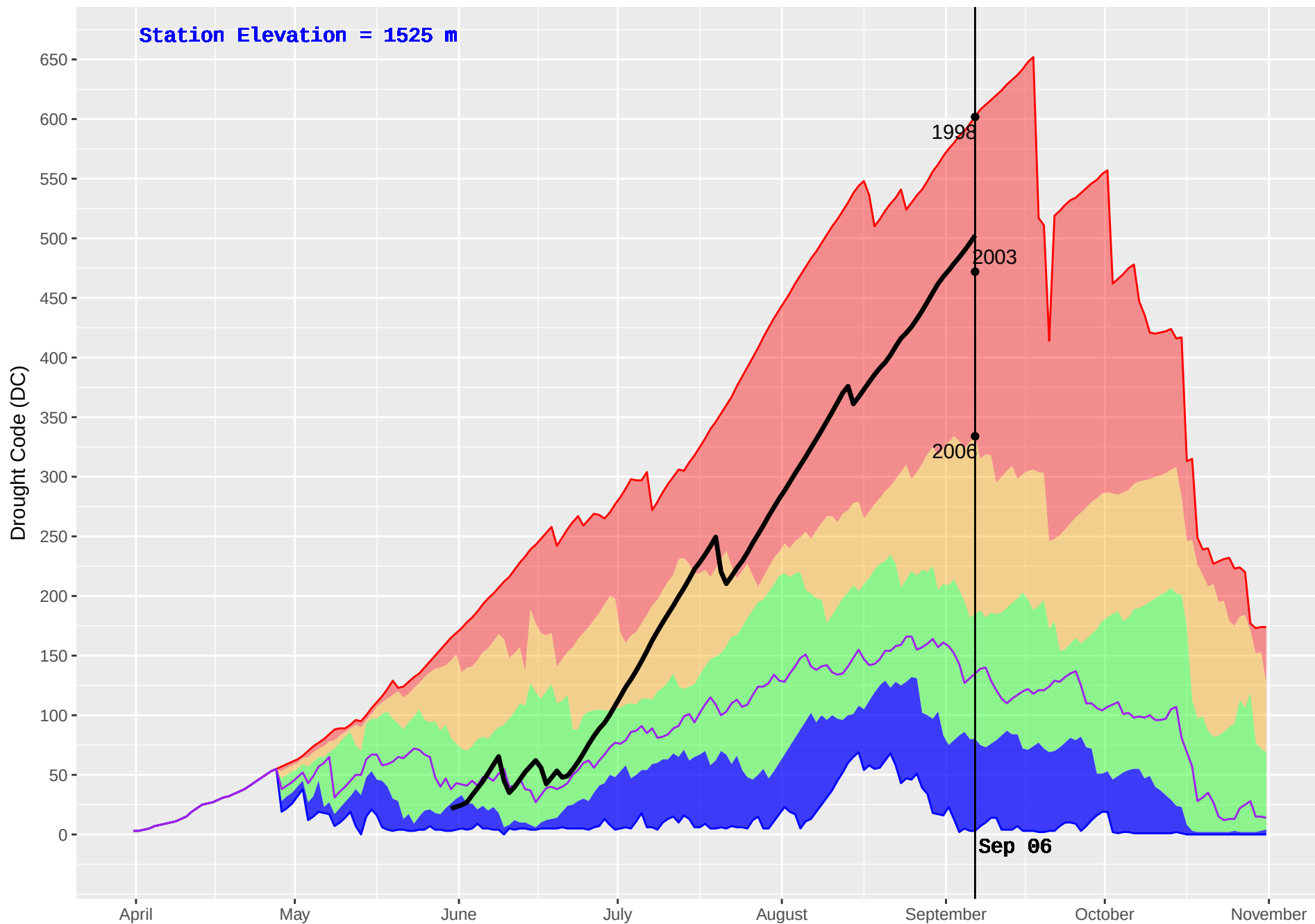
HARBOUR LAKE (250) : Historical (1989–2016) and Current (2017) Noon Drought Code (DC)
